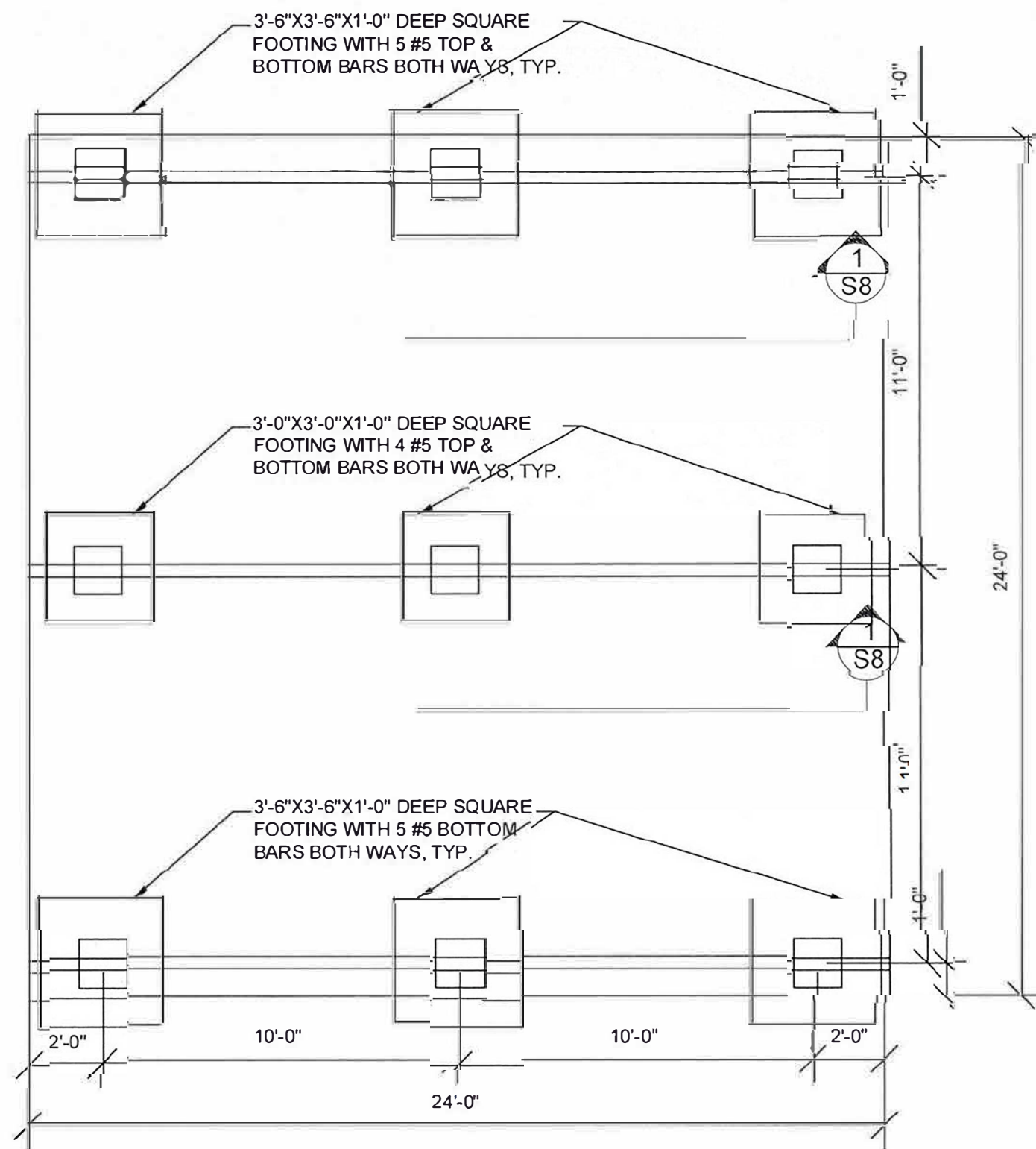
1 FOUNDATION PLAN DO NOT SCALE DRAWING
